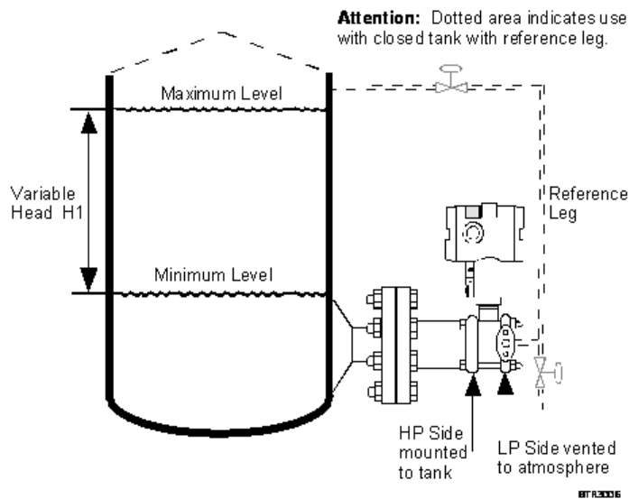
Figure 3 – Typical mounting for flange mounted level transmitter
